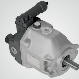
WINMAN axial verstellkolbenpumpe WINMAN variable axial displacement piston pump
