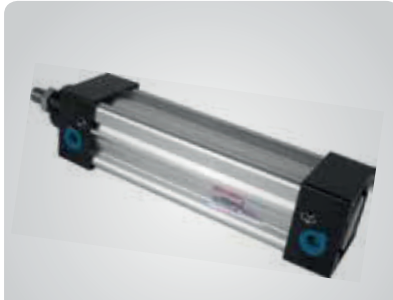
WINMAN WSI-M-YY ISO 15552 serie pneumatikzylinder WINMAN WSI-M-YY ISO 15552 series cylinders
